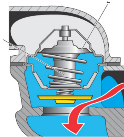
Fig. 5-19 Termostato cerrado
